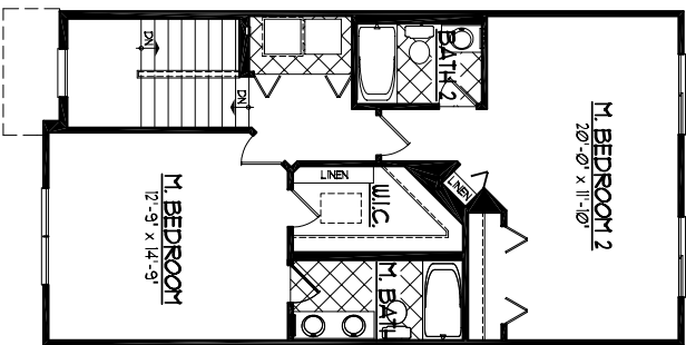
PART'L SECOND FLOOR PLAN w/ OPT'L DELUXE M. BATH
