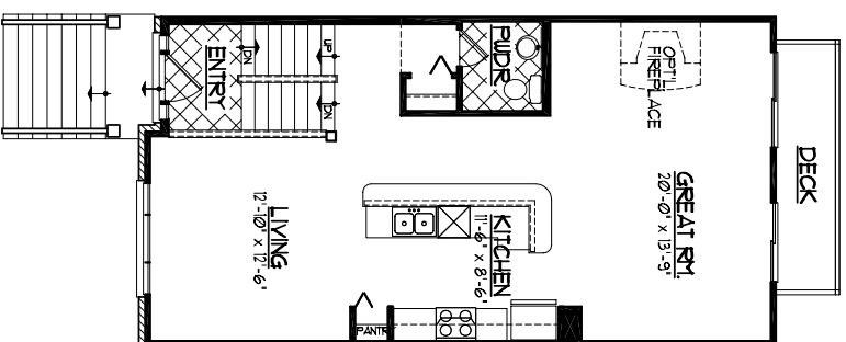
FIRST FLOOR PLAN w/ CITY LOFT OPTION
