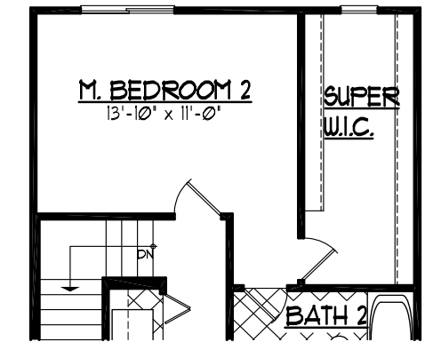
PART'L. SECOND FLOOR PLAN w/ OPT'L SUPER WIC
