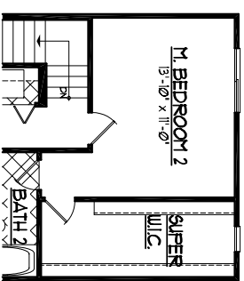
PARTIAL SECOND FLOOR PLAN w/ OPT. SUPER WIC
